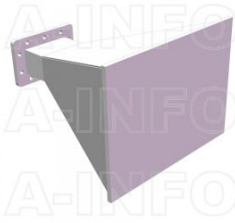
LB-284-15-ASPO Standard Gain Horn Antenna 2.6-3.95GHz 15dB Gain Rectangular Waveguide Interface
