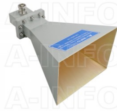
LB-284-15-C-7/16F Standard Gain Horn Antenna 2.6-3.95GHz 15dB Gain 7/16(DIN) Female
